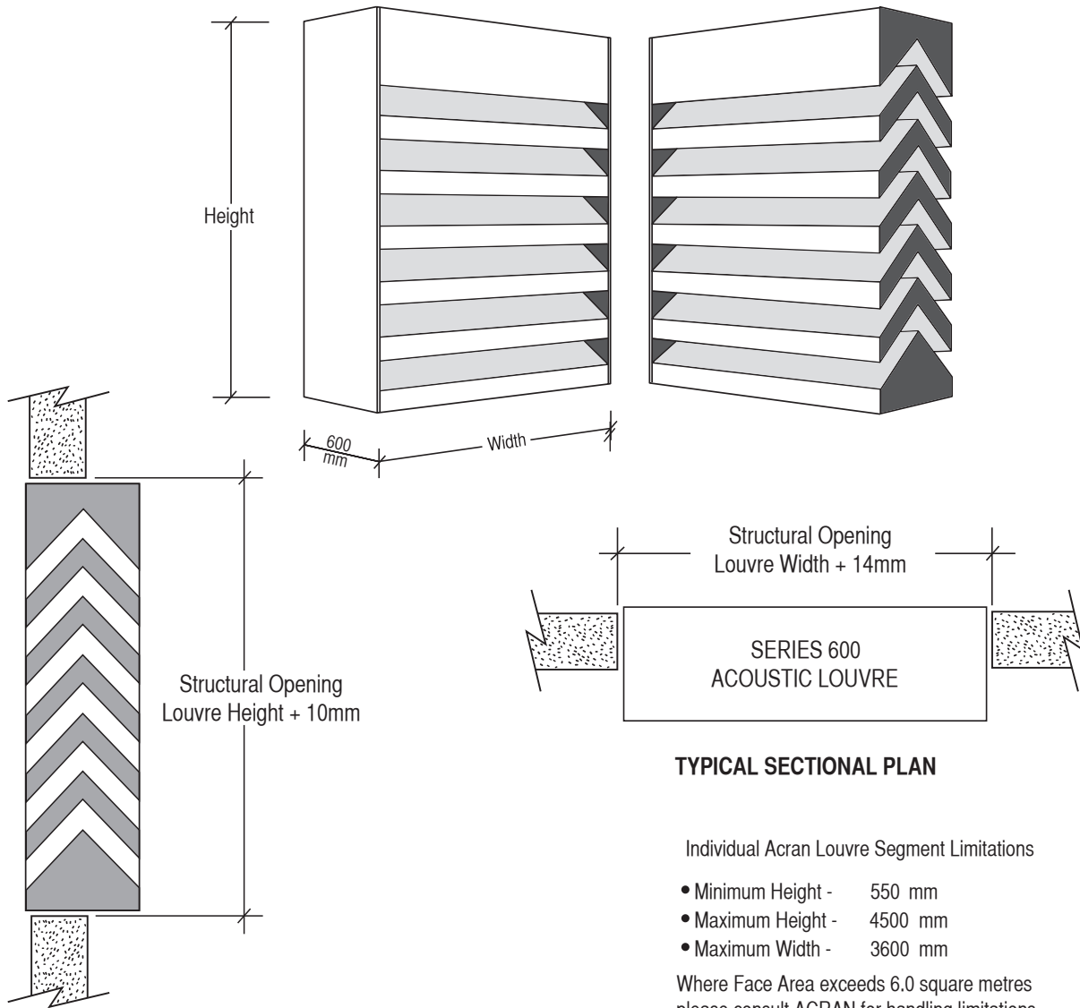
TYPICAL SECTIONAL ELEVATION
