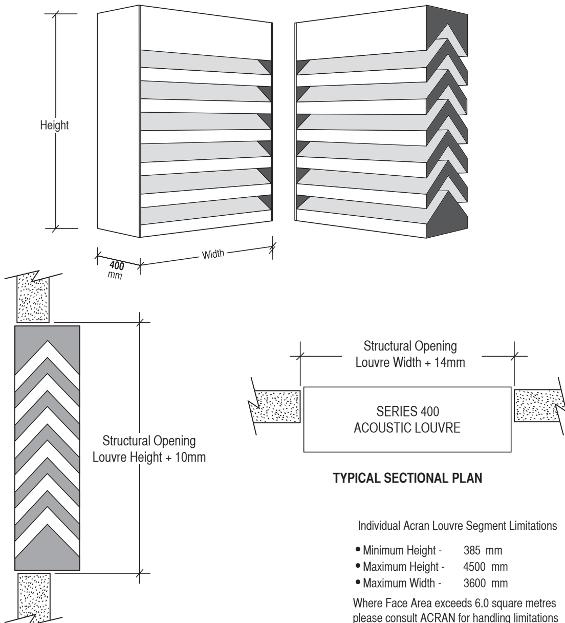
TYPICAL SECTIONAL ELEVATION
