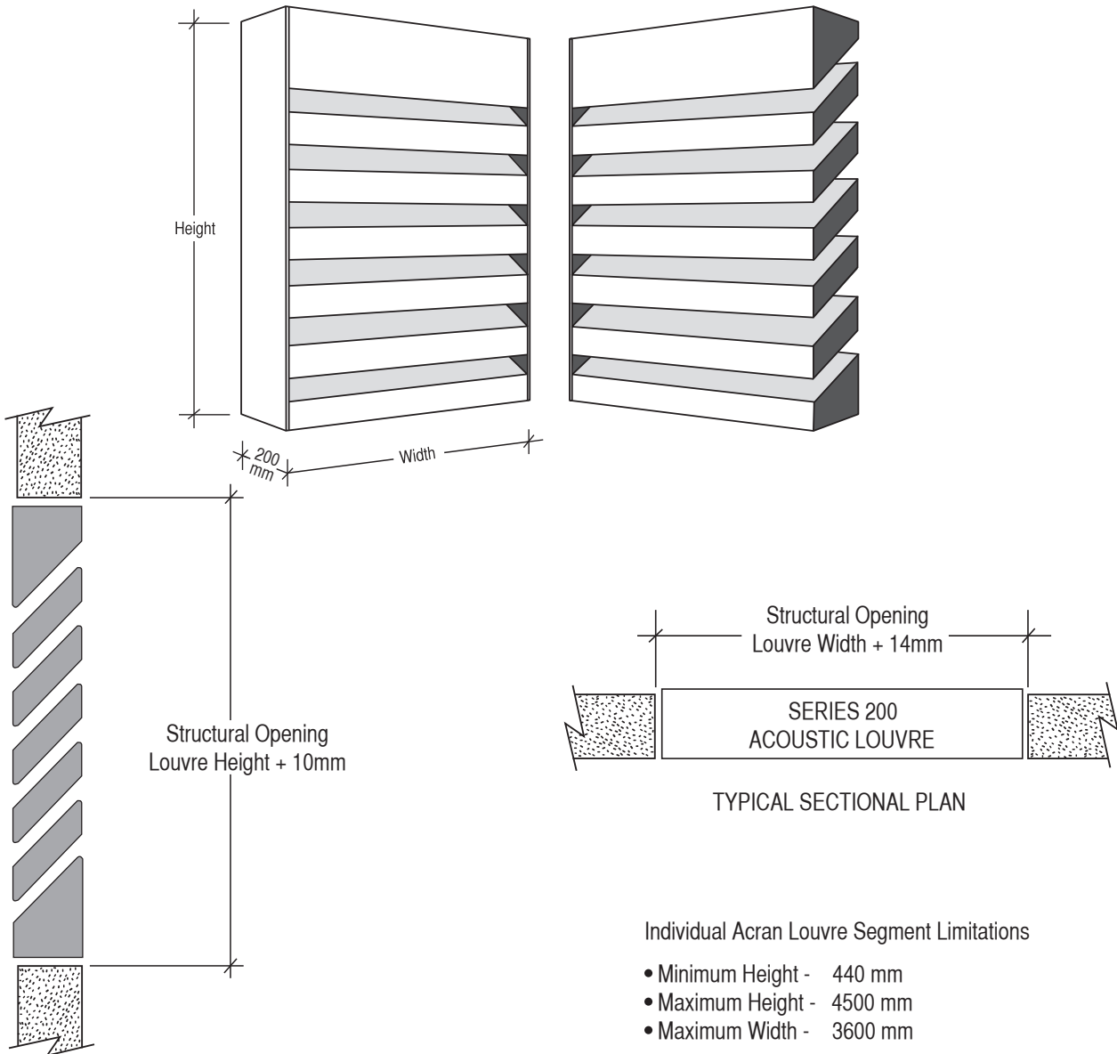
TYPICAL SECTIONAL ELEVATION
