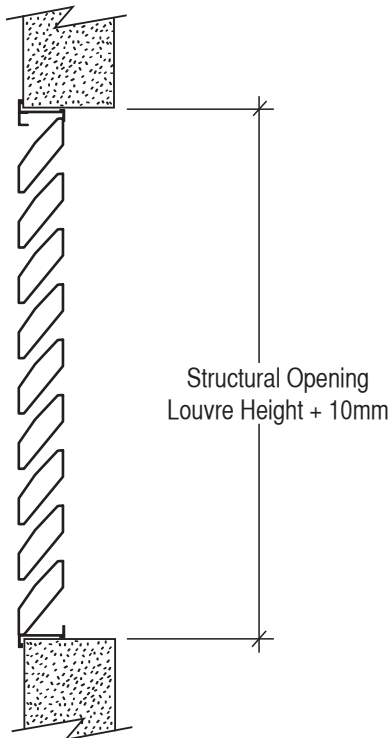
TYPICAL SECTIONAL ELEVATION
